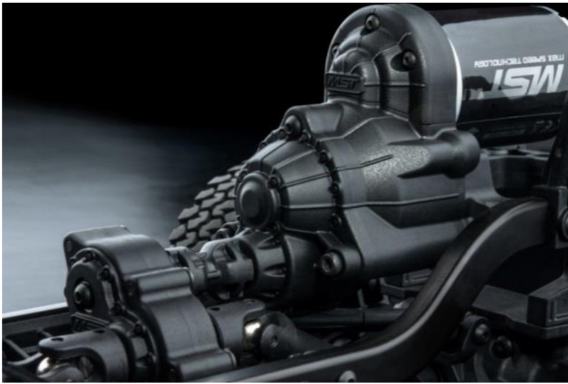
Front motor with the planetary gearbox
